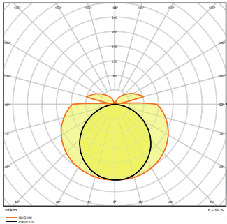
LDVAL BAT HE 1200 13W G3 24X1 EN LEDV
